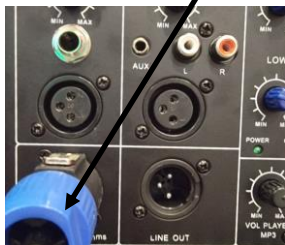
Powered Speaker Input
